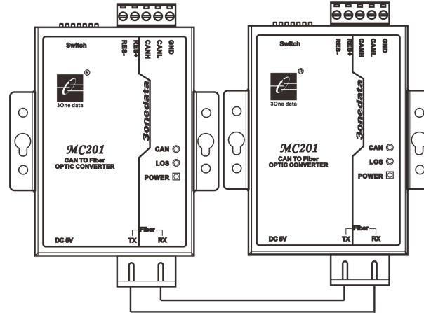
MC201 Fiber Interface connection diagram
